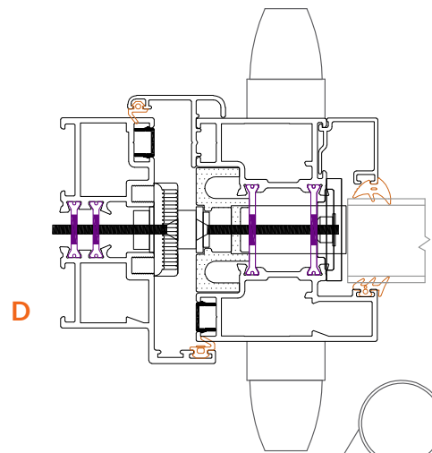
Traditional lock detail
