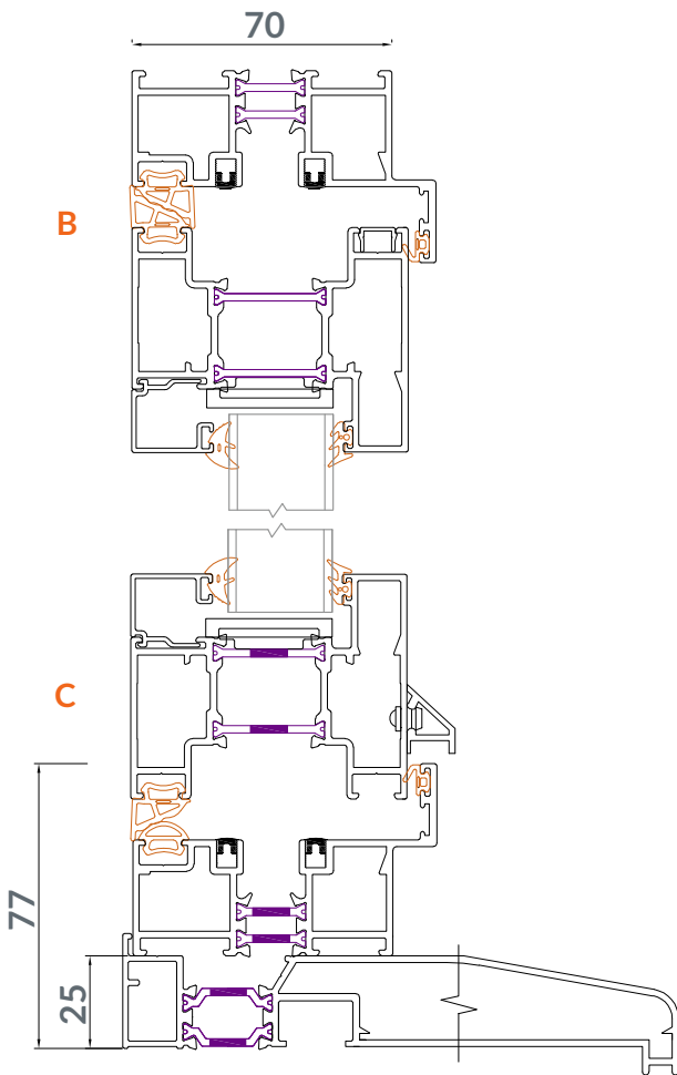
Cill and threshold detail
