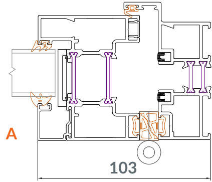
Frame and sash detail
